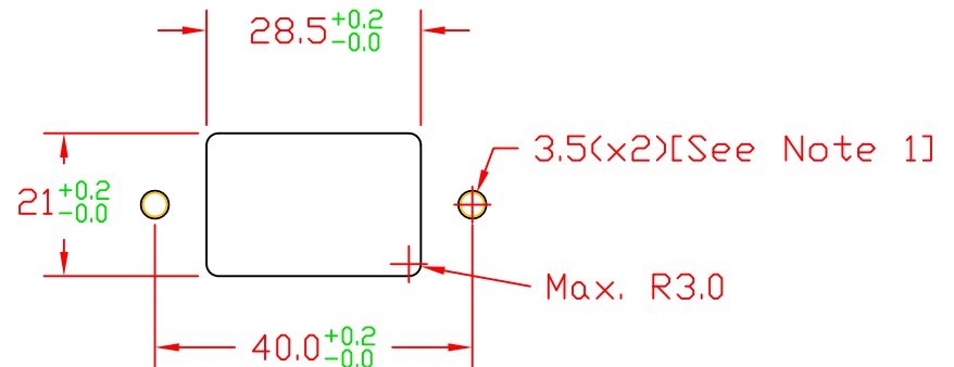
Rear-side mounting
