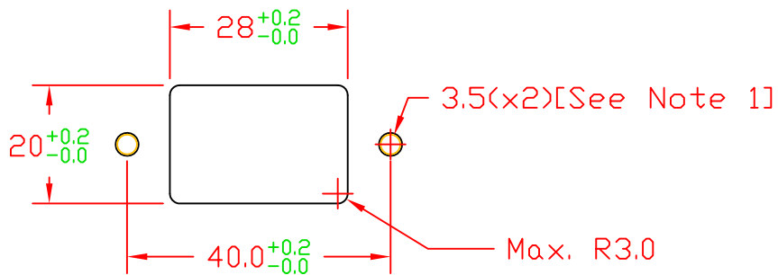
Front-side mounting
