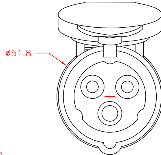
END VIEW (SHOWN WITH LID OPEN)
