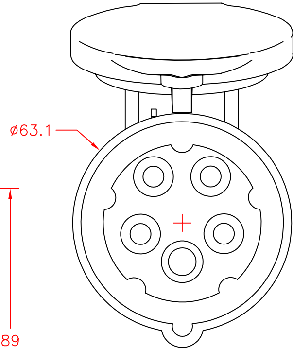
END VIEW (SHOWN WITH LID OPEN)
