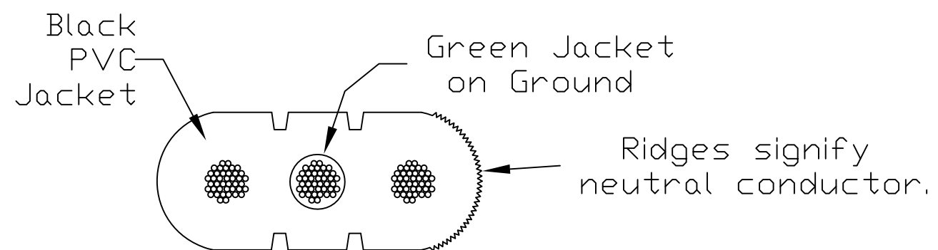
CROSS-SECTION OF CABLE ENLARGED VIEW
