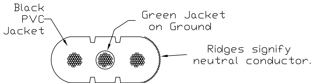
CROSS-SECTION OF CABLE ENLARGED VIEW
