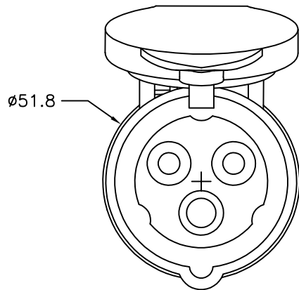
END VIEW (SHOWN WITH LID OPEN) 6 HOUR
