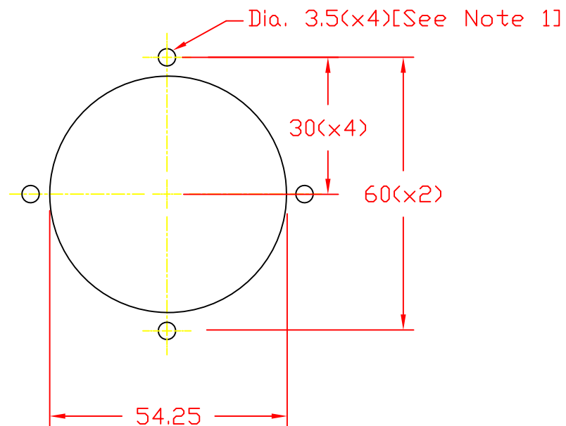
MOUNTING HOLE
