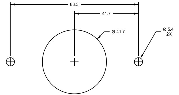
SUGGESTED CUTOUT
