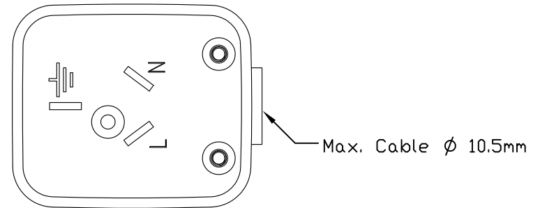
FACE VIEW
