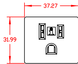
88221100 & 88222100 QUICK DISCONNECT CONTACTS
