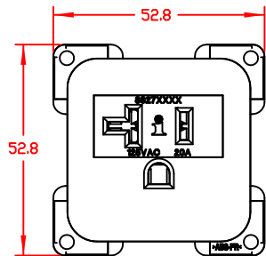
8827100 & 88272100 QUICK DISCONNECT CONTACTS
