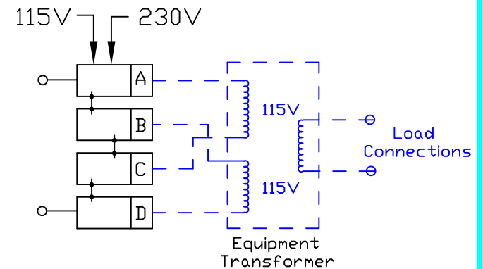
Modules with a Voltage Selector
