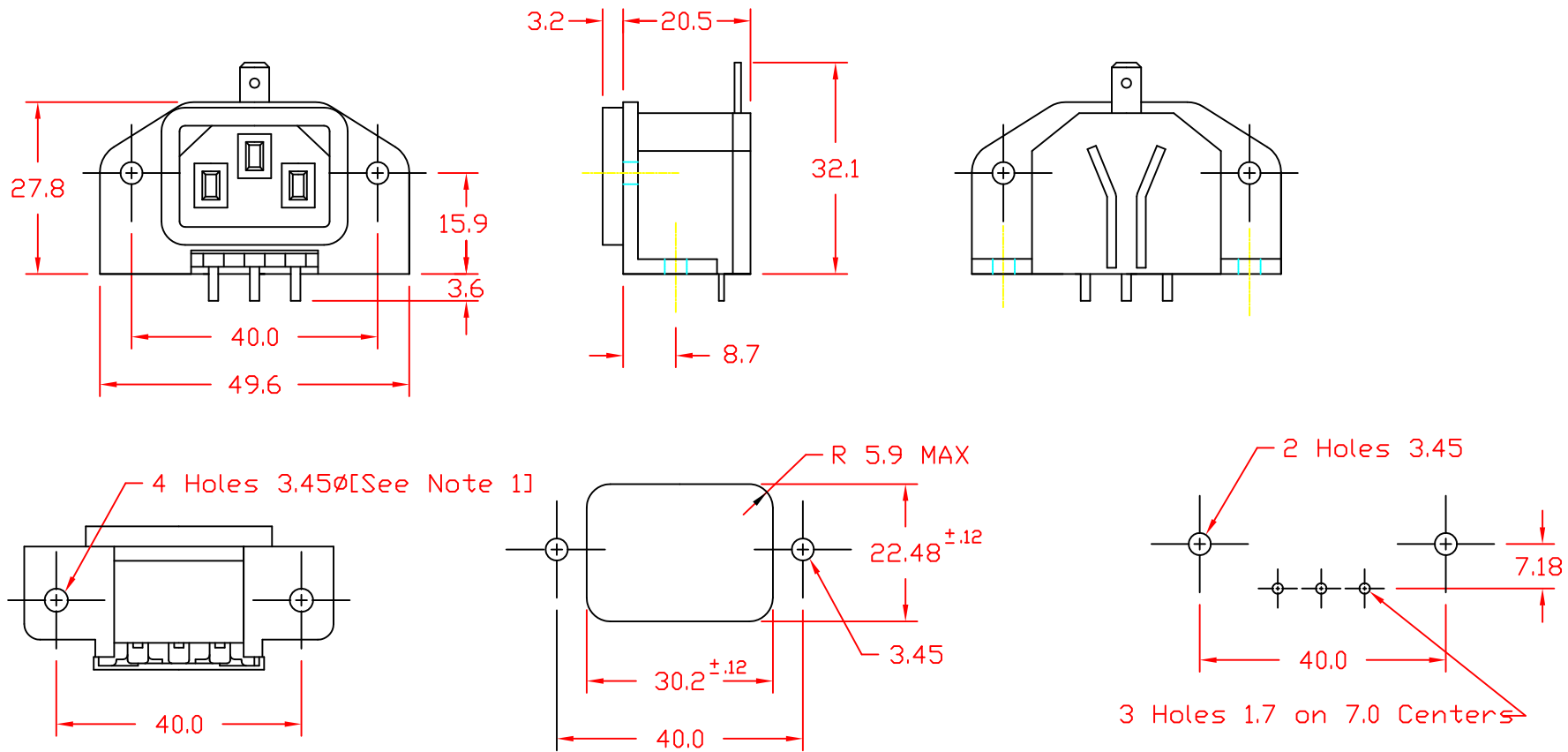
PCB MOUNTING DETAIL
