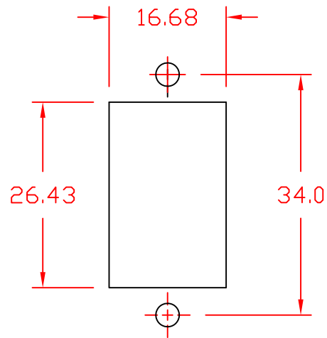
Cut-out for mounting switch on surface
