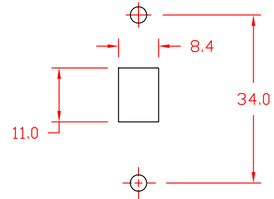
Cutout for mounting switch behind panel
