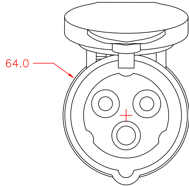
END VIEW (SHOWN WITH LID OPEN)
