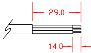
Strip Length
